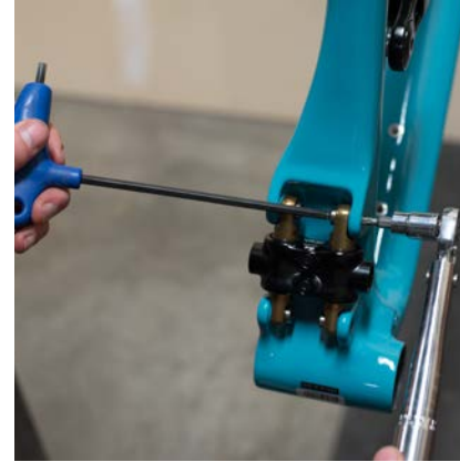
09. Use a ball-end wrench to prevent the inner Ti Female Bolts from rotating. Torque the 4x Flat Head Ti Male Bolts to 12 Nm .
